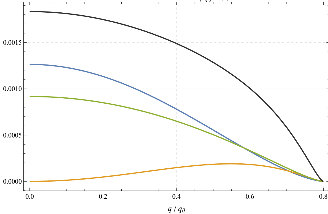
Kernel Functions for M / q_0 = 0.3
